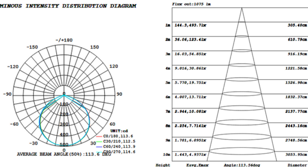
LUMINOUS INTENSITY DISTRIBUTION DIAGRAM
